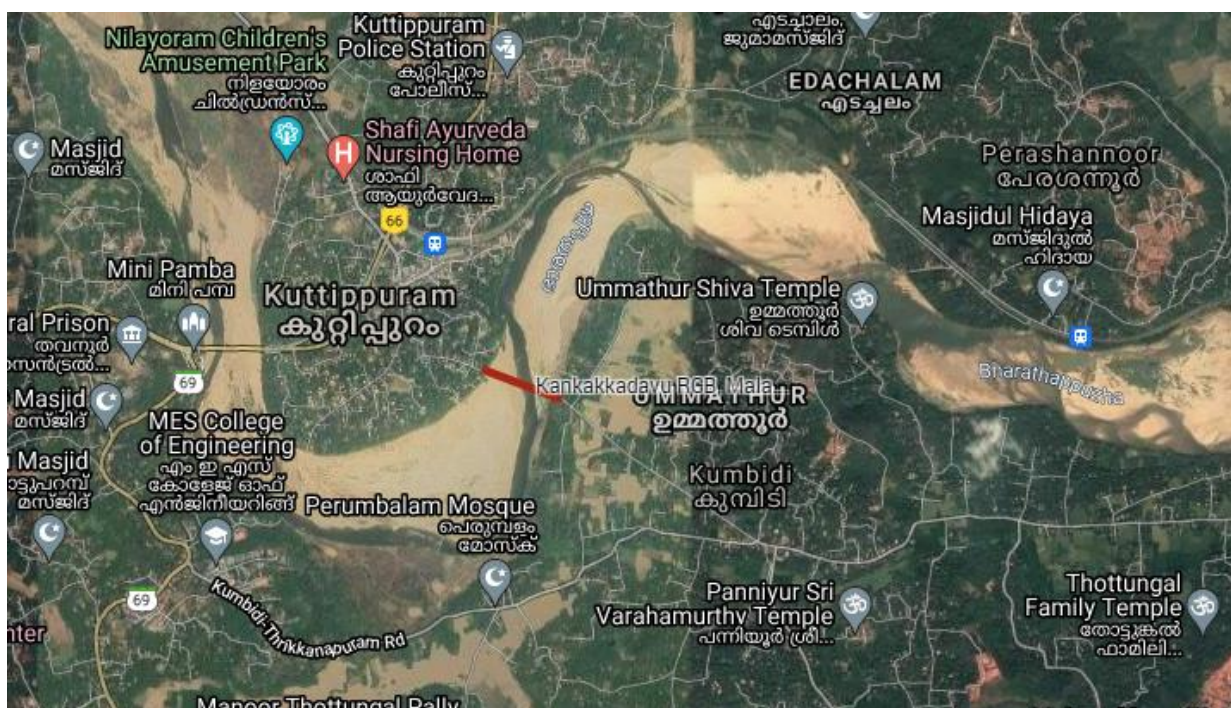
Figure 1.1: Proposed location of the regulator cum bridge
